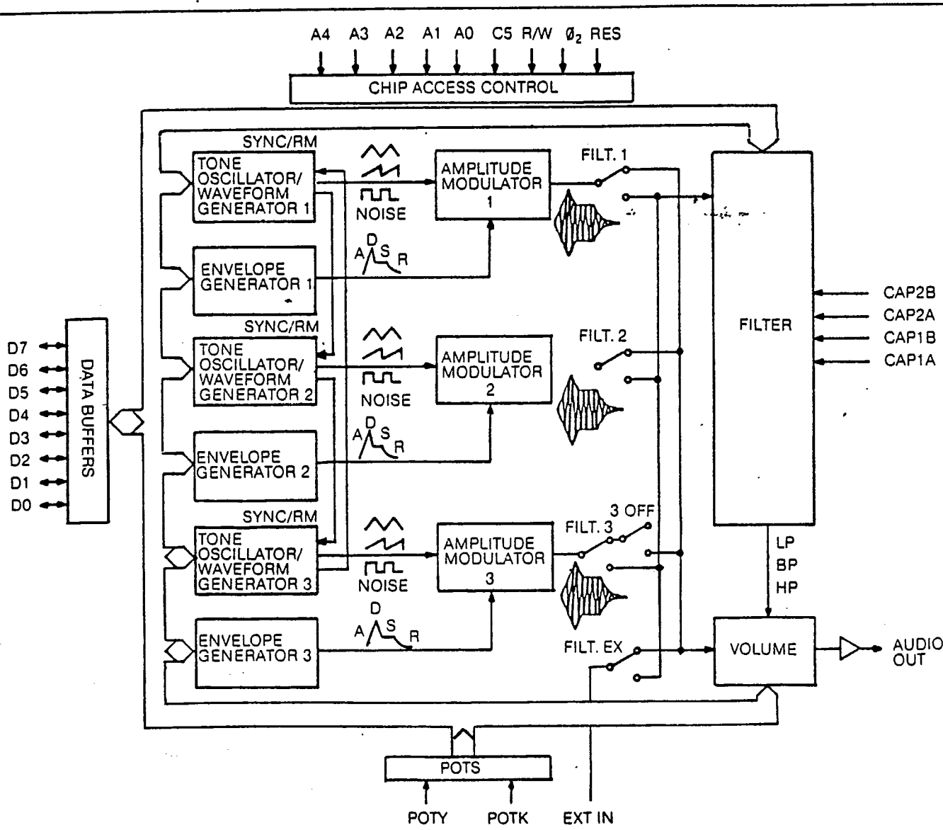
6581 SID BLOCK DIAGRAM
